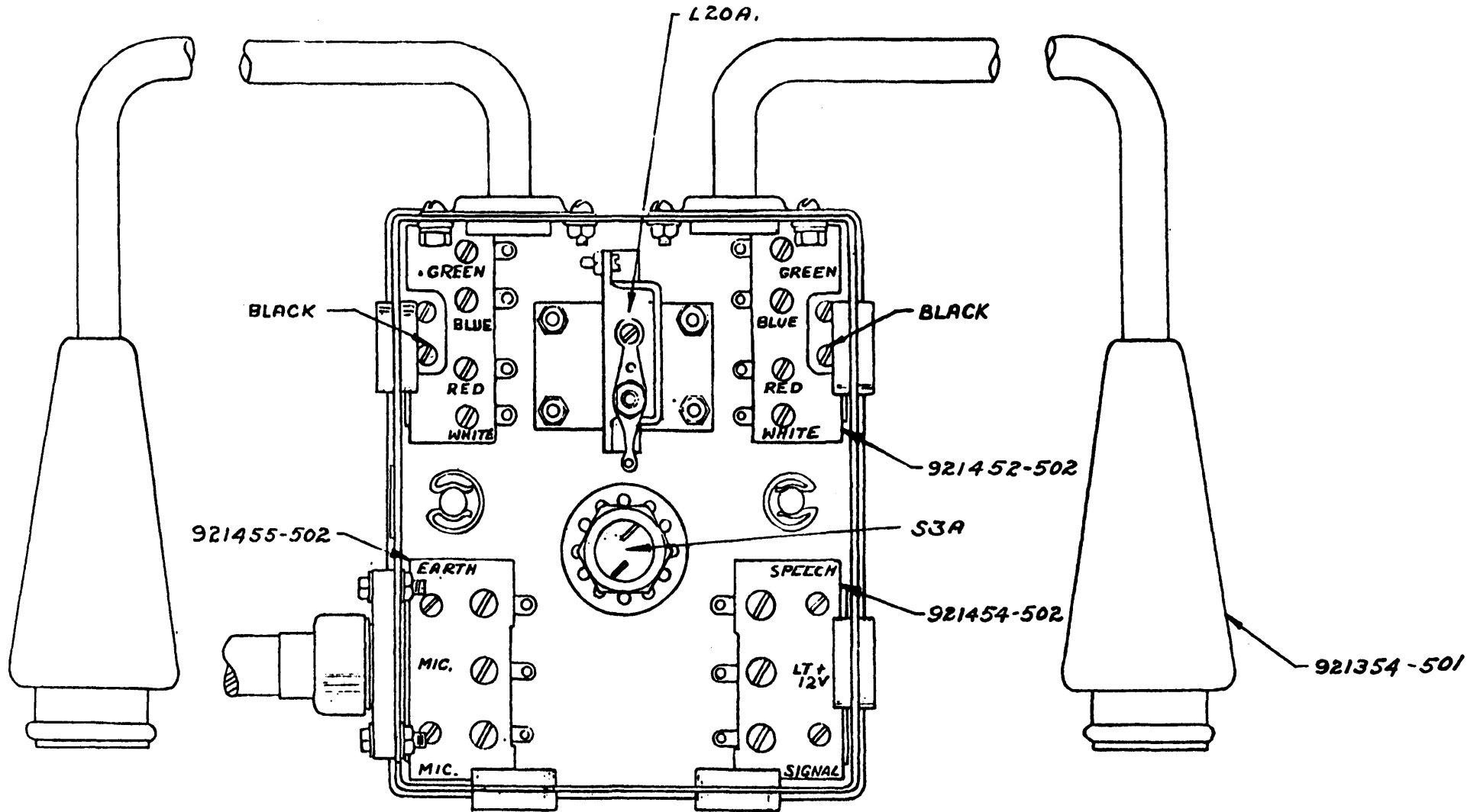
BOTTOM VIEW
