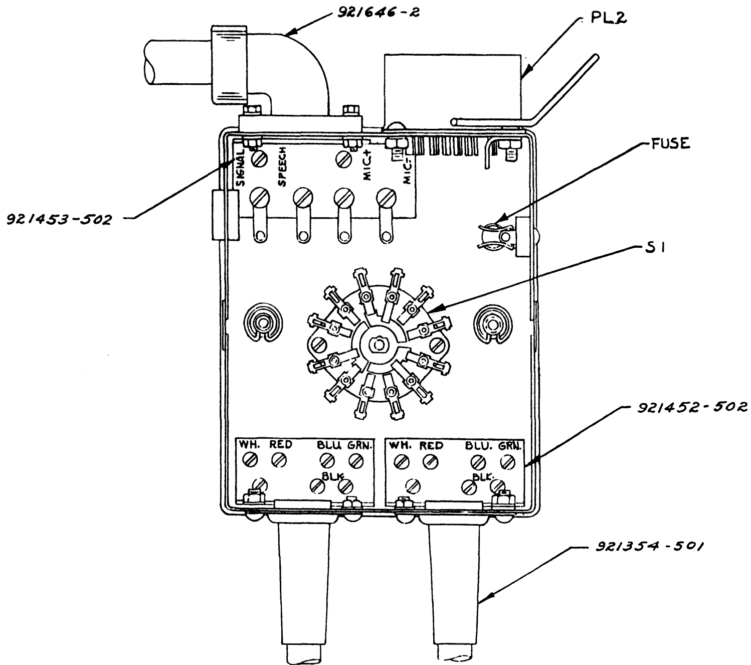
CONTROL UNIT N°1 MK. II
