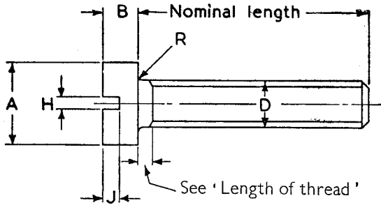
Cheese head screw
